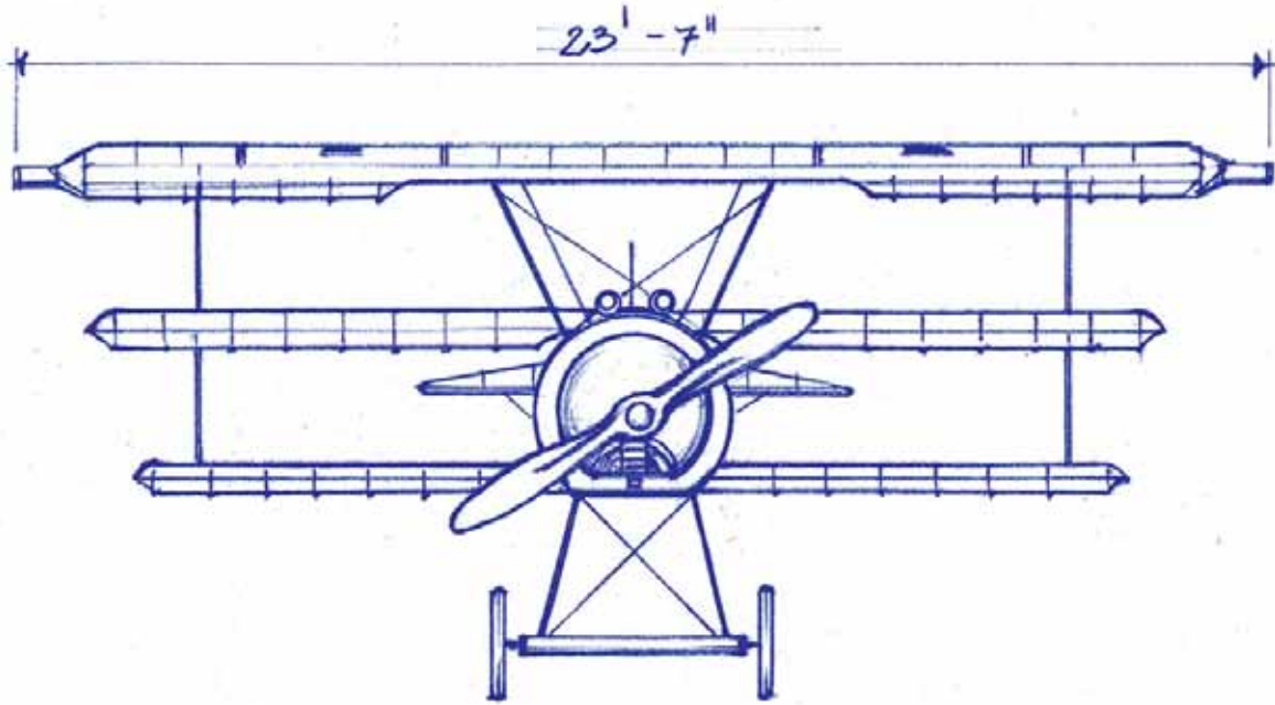
FRONT VIEW
