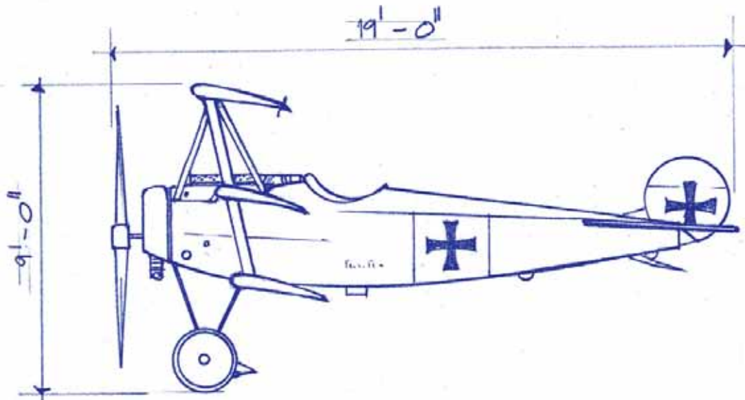
SIDE VIEW
